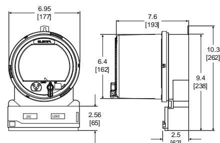
Dimensions in inches [millimeters]. For reference only.
