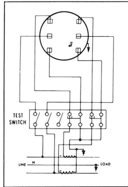
SINGLE PHASE 3 WIRE
