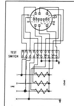
3 PHASE 4 WIRE "Y" USING CT'S
