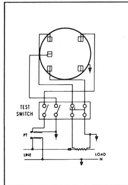
SINGLE PHASE 2 WIRE CT AND PT
