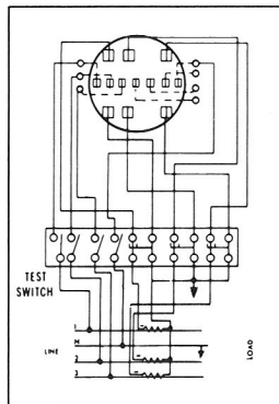
3 PHASE 4 WIRE Δ USING CT'S
