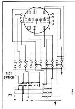
3 PHASE 4 WIRE "Y" USING CT'S & PT'S
