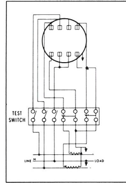
3 PHASE 3 WIRE WITH CT'S AND PT'S OR NETWORK
