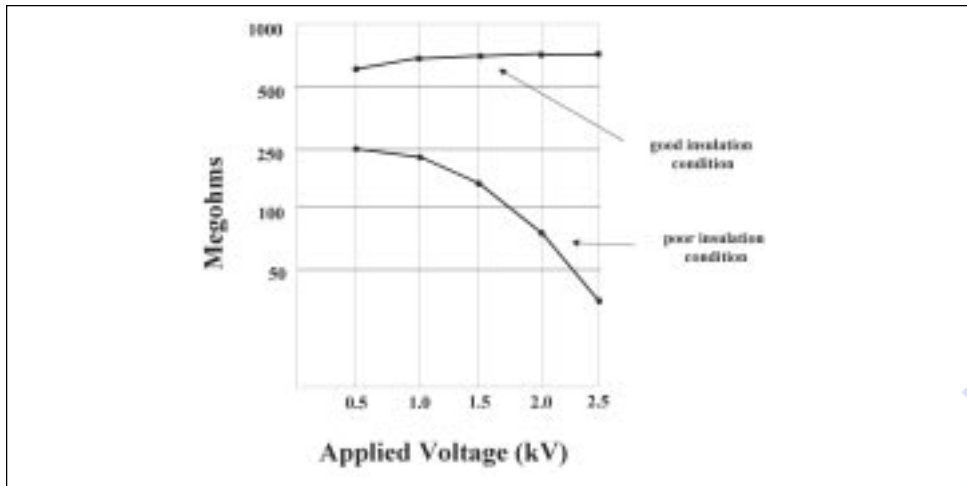
Figure 15: Step Voltage Step Graph
