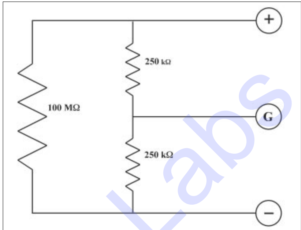
Figure 19: Guard Terminal Diagram
